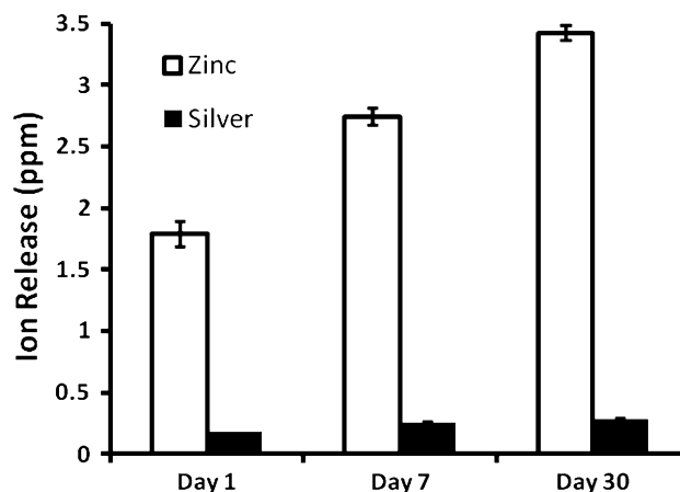
Fig. 2 Cumulative ion release profiles for Zinc and Silver from the GPC
