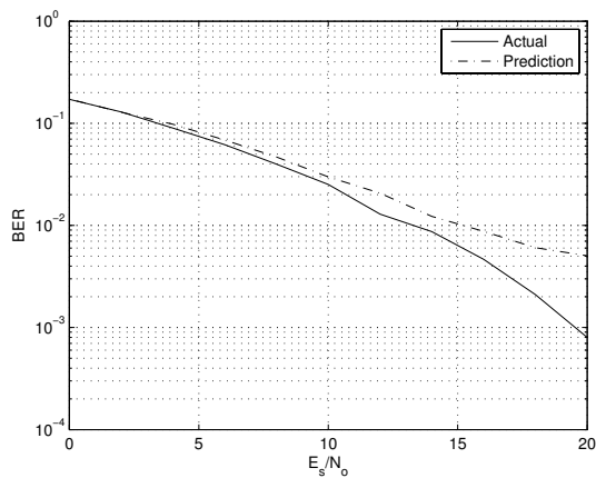
Fig. 11. BER for a un-coded 2 \times 2 MIMO fast fading channel.
