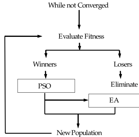
Fig. 3. PSO-EA algorithm.
