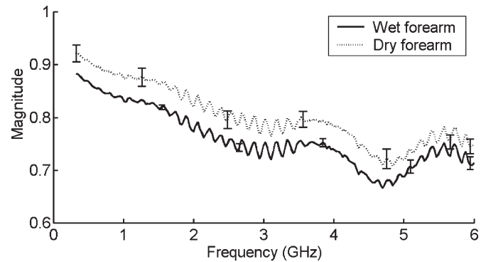
Fig. 8. Effect of prolonged soaking of forearm skin on the magnitude of reflection coefficient.
