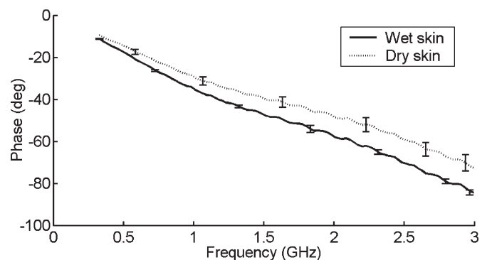
Fig. 5. Effect of prolonged skin soaking on the phase of reflection coefficient.
