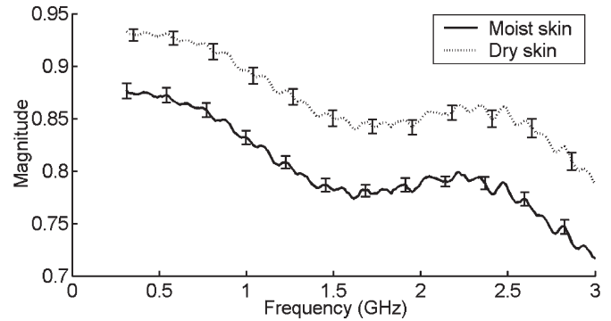
Fig. 4. Effect of prolonged skin soaking on the magnitude of reflection coefficient. Note that the difference in reflectance magnitude, about 0.06 , remains fairly constant across all measured frequencies.
