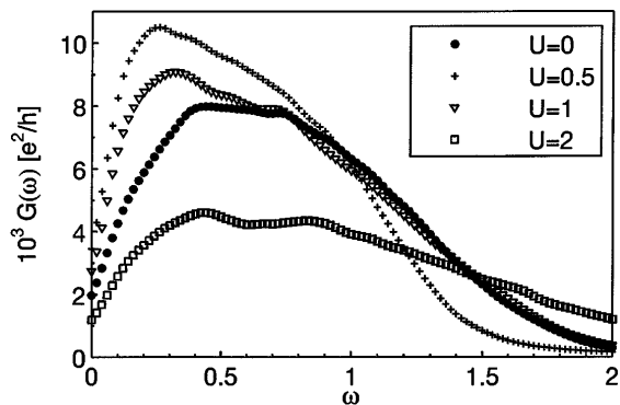
FIG. 3. G(\omega) for W = 1 , t = 0.03 , \gamma = 0.05 .
