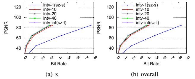
Fig. 5. Rate distortion of SZST on EXAALT
