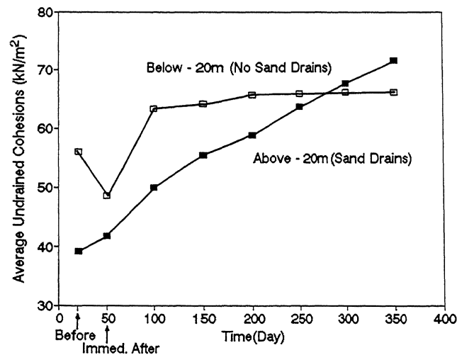
Fig. 9 Average undrained cohesion with various time intervals
