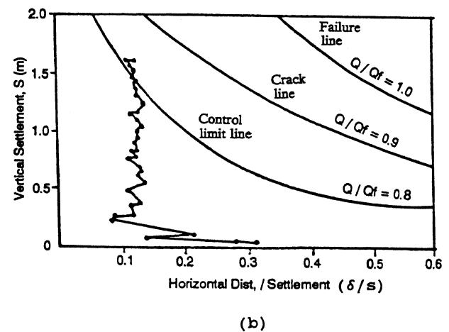
Fig. 6 Field observation of the settlement, (a) typical staged construction process for preloading, and (b) stability control method for the hot strip mill site
