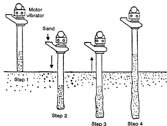
Fig. 3 Construction sequence for sand drains
