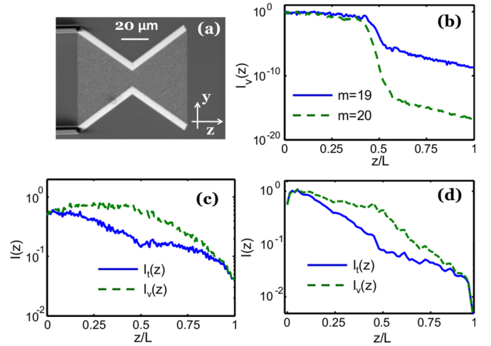
FIG. 6. (Color online) Transmission eigenchannels and intensity decay in a diffusive waveguide of bow-tie geometry. (a) Top-view SEM image of a fabricated quasi-2D waveguide with bow-tie geometry. The length of waveguide is L = 80 \mu\text{m} . The width of waveguide decreases linearly from 60 \mu\text{m} at z = 0 to 10 \mu\text{m} at z = L/2 and then again increases linearly to 60 \mu\text{m} at z = L . (b) Numerically calculated cross-section-averaged intensity I_v(z) of the 19th (solid line) and 20th (dashed line) transmission eigenchannels of bow-tie waveguide. The length L of the waveguide is 20 \mu\text{m} , the width at z = 0, L is 10.2 \mu\text{m} (35 propagating modes) and the width of constriction at z = L/2 is 5.1 \mu\text{m} (17 propagating modes). The abrupt changes in the decay rate of I_v(z) before and after z = L/2 indicate the conversion from propagating wave to evanescent wave and back. The evanescent decay rate varies from one channel to another. (c) Numerically-calculated I_v(z) (green dashed line) and cross-section-integrated intensity I_t(z) (blue solid line) for the maximum transmission channel of the same waveguide as in (b) but with absorption L/\xi_a = 3 . The constriction causes a significant change in the intensity distribution of the maximum transmission channel. (d) Experimentally measured I_v(z) (green dashed line) and I_t(z) (blue solid line) inside the disordered waveguide shown in (a). Both intensity distributions follow those of the maximum transmission channel.
