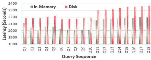
FIGURE 13. Mean latency per query for 1 million smart meters across 1-Node.
