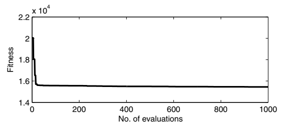
Fig. 3. Convergence of the proposed BFT with PSO biased evolution.
