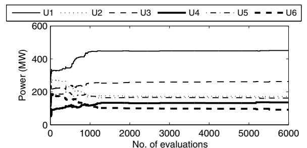
Fig. 1. Movement of the best bacterium (6-unit system).
