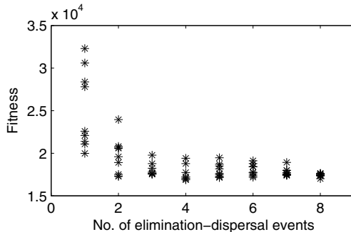
Fig. 2. Swarm behavior.
