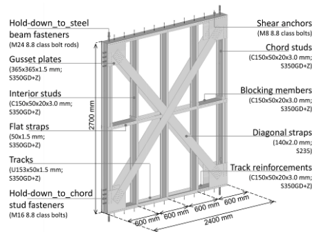
Figure 2. WHD wall configuration
