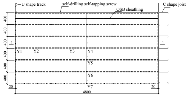
(a) layout of specimen FL-1
