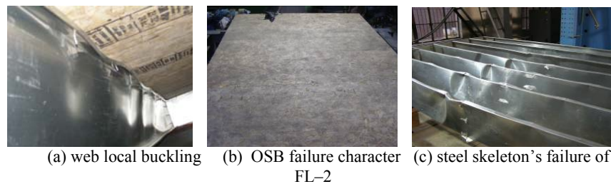
Figure 4 Failure characteristics of composite floor
