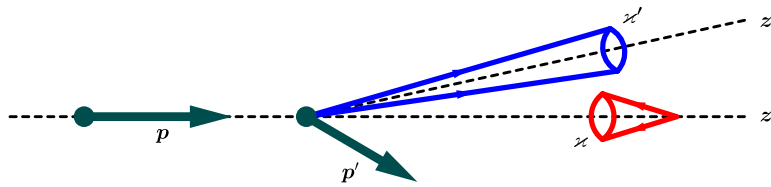
Fig. 3 (Color online) Schematic view of the scattering geometry. The incoming twisted photon with transverse momentum spread \mathcal{K} is scattered by a counterpropagating electron with momentum p , into a state propagating along an arbitrary z' axis with transverse momentum
