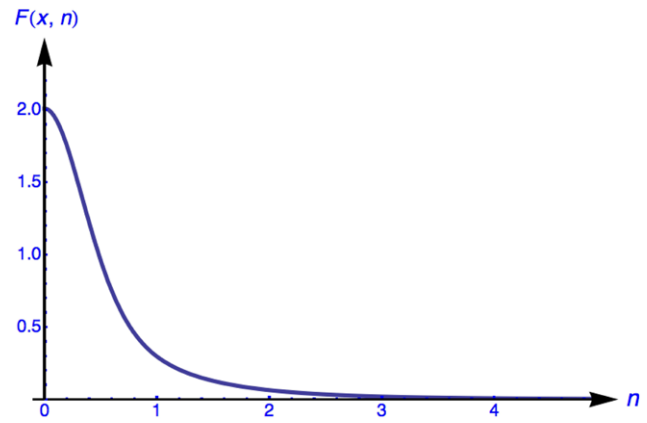
Fig. 4 The angular distribution d\sigma/d\Omega' = 2\alpha^2 \gamma^2 m_e^{-2} F(x, n) of the final photons in the Compton scattering in dependence on n = \gamma\theta' . The value x = 0.092 corresponds to the VEPP-4M collider
