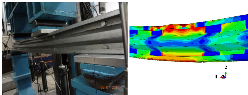
(b) Distortional buckling
