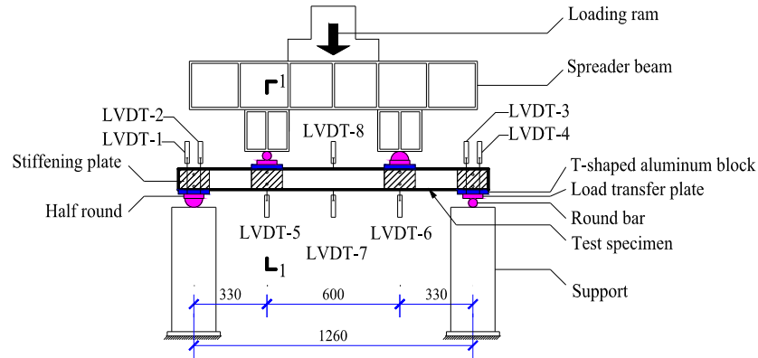
Figure 3: Schematic view of four-point bending test arrangement
