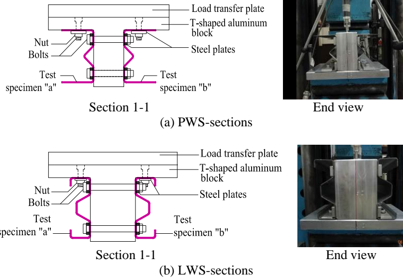
Figure 5: Details of the T-shaped aluminum load transfer blocks at loading points and end supports
