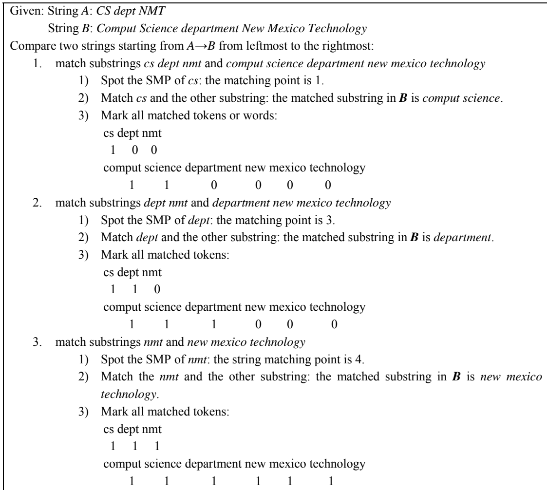
Figure 1. An example of string matching using the concept of string matching points.
