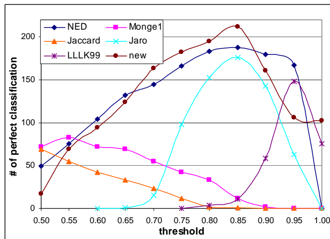
Figure 5. Perfect classification results using different field matching algorithms.
