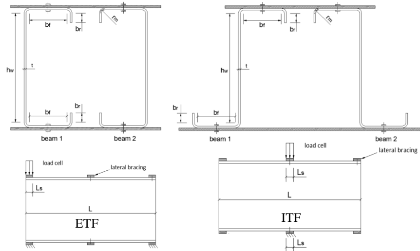
Fig. 4. Group (iv) by Beshara and Schuster (2000)
