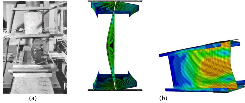
Fig. 7: (a) Failure of I-6-ETF-1 – Group (i) (Hettrikul and Yu 1978), (b) SFE model
