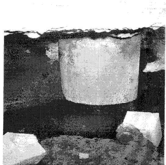
Fig. 7. Undamaged pile under ferry building in Port Island after Kobe earthquake, 1995.
