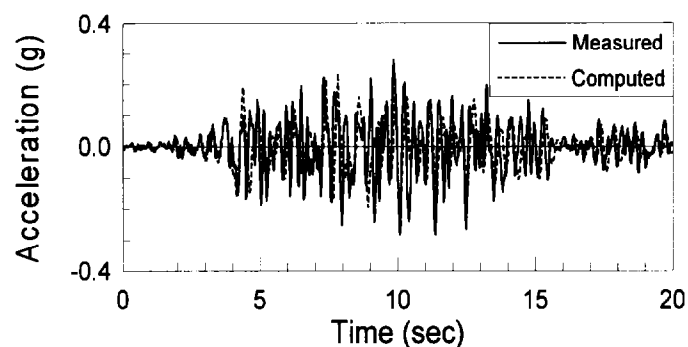
Fig. 27. Comparison of measured and computed pile cap acceleration time histories.
