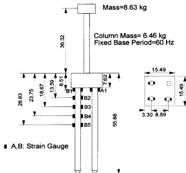
Fig. 19. Instrumented pile for single pile test.
