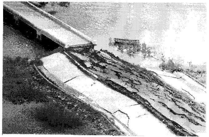
Fig. 5. Bridge on undamaged pile foundations with failed embankment; Nihon-kai-chubu earthquake, 1983.
