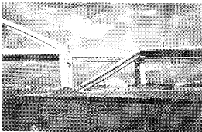
Fig. 10. Collapse of the deck of Nishinomiya bridge during the Kobe earthquake
