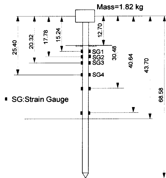
Fig. 19. Instrumented pile for single pile test.
