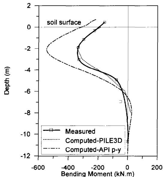
Fig. 14. Comparison of measured and computed bending moments.
