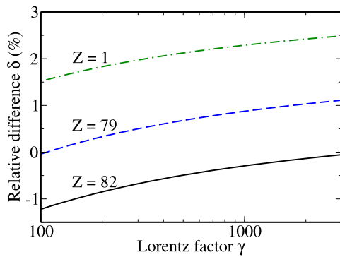
Fig. 2 The relative difference (55) between rigorous relativistic results and predictions of the scaled EPA–Sauter approximation (54) for the total cross sections of bound–free pair production. Calculations are performed for the energetic collisions between two protons (dash-and-dotted line) as well as bare gold Au 79+ (dashed line) and lead Pb 82+ (solid line) ions. The EPA–Sauter cross section is given by Eqs. (50) and (51) derived using a value of Q_{\max}^2 = 4m^2 (Color figure online)
