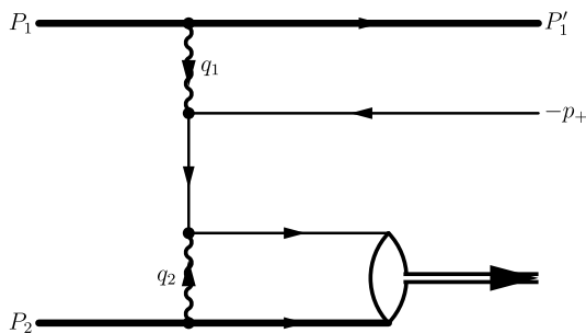
Fig. 1 Schematic Feynman diagram for the bound–free pair production in a heavy-nucleus collision. Heavy colliding nuclei are represented by thick lines while thinner lines correspond to light fermions (electron and positron). The trajectory of the produced electron is aligned with that of the second nucleus
