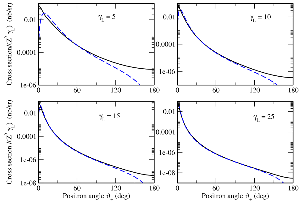
Fig. 4 The differential cross section (Z^5\gamma_L)^{-1}d\sigma_{\gamma Z}/d\Omega_+ (in nanobarn/steradian) of the pair production in the collision of photon with bare lead Pb^{82+} ion accompanied by the electron capture into the ground ionic state. Results of the rigorous relativistic calculations ( solid line ) are compared to the predictions of the scaled Sauter approximation ( dashed line ). Calculations have been performed in the nucleus rest frame and four positron energies m\gamma_L with \gamma_L = 5, 10, 15 and 25 (Color figure online)
