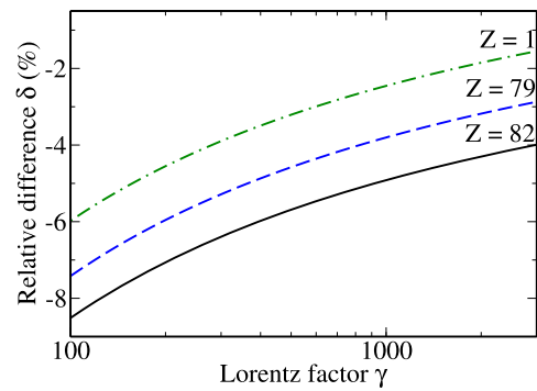
Fig. 3 The same as in Fig. 2, but the EPA–Sauter cross section is given by Eqs. (50) and (52) employing a value of Q_{\max}^2 = 1.26m^2 (Color figure online)
