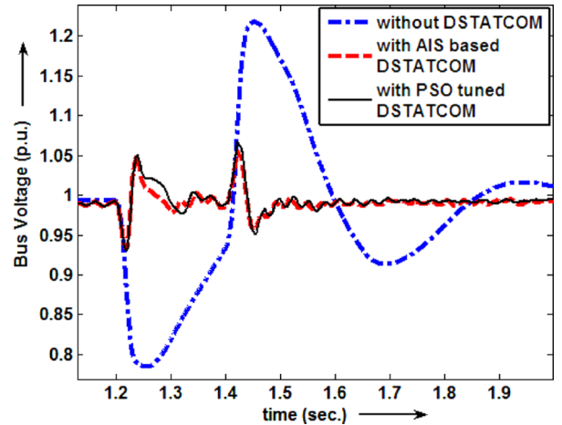
Fig. 7. Performance comparison for pulse load of 20 MW/40 MVAR for 200 ms.
