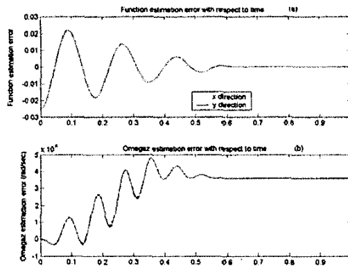
Fig. 1. Functional and rate estimation error.
