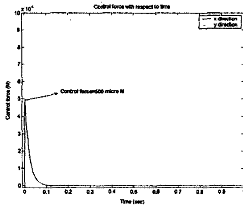
Fig 3. Control input without magnitude constraints.
