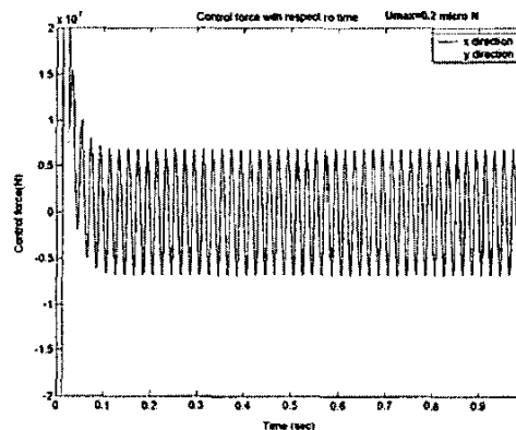
Fig 2. Control input with magnitude constraints.
