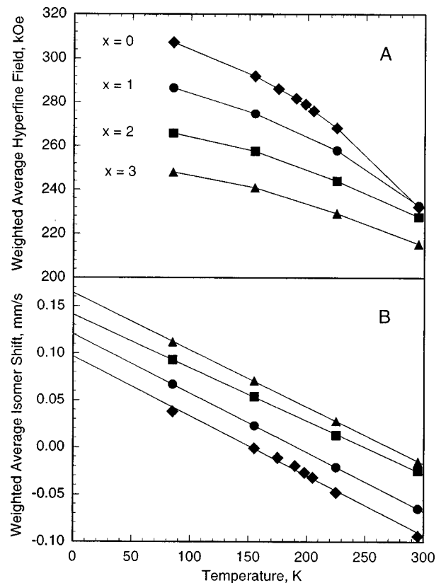
FIG. 3. The temperature dependence of the weighted average hyperfine fields, A, and the weighted average isomer shifts, B, for the Tb_2Fe_{17-x}Si_x solid solutions with x = 0, 1, 2, and 3 .
