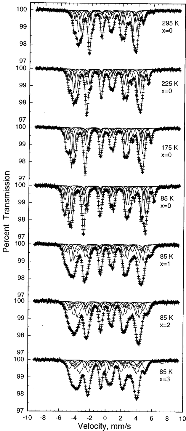
FIG. 1. The Mössbauer spectra of Tb_2Fe_{17} measured at 295, 225, 175, and 85 K, and the 85 K Mössbauer spectra of the Tb_2Fe_{17-x}Si_x solid solutions with x = 1, 2, and 3 .
