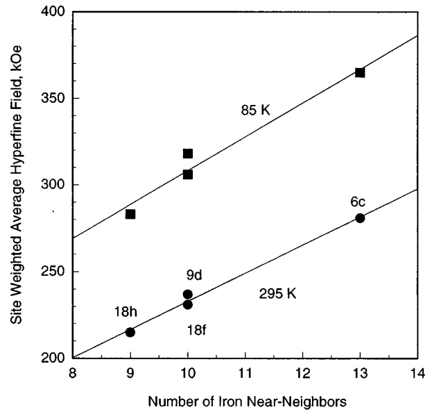
FIG. 2. The correlation between the Tb_2Fe_{17} site weighted average hyperfine fields and the number of iron near-neighbors.
