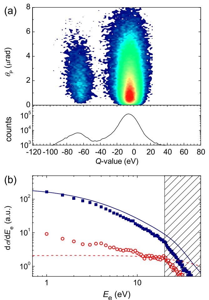
FIG. 2 (color online). (a) Cross sections of single ionization in 1.5 MeV/u O^{8+} -Li collisions as a function of the Q -value and the projectile scattering angle \theta_p . (b) d\sigma/dE_e (a.u.) of the same collision system for pure 2s ionization (solid squares) and ionization-excitation (open circles). The curves are CDW-EIS results for 2s (solid line) and 1s (dashed line) ionization. In the shaded range a significant fraction of the electrons is not detected due to acceptance limitations.
