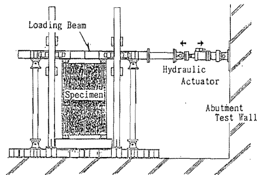
Fig.4 Loading Setup
