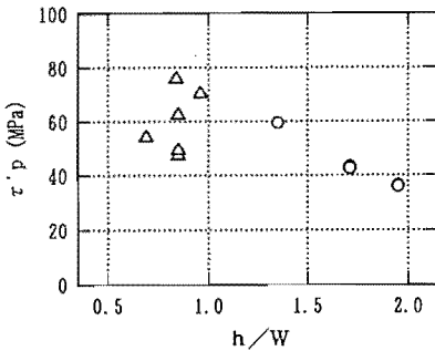
Fig.16 Ultimate Plastic Strength
