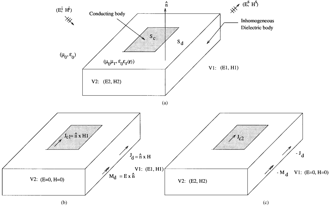
Fig. 2. Geometry of an inhomogeneous dielectric body partially covered by conductors: (a) the original problem, (b) its external equivalence, and (c) internal equivalence.
