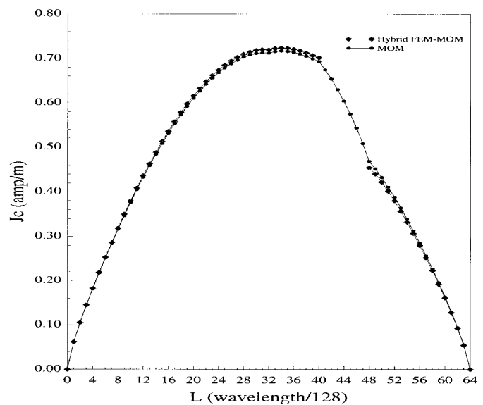
Fig. 10. Dipole current distribution in the presence of a dielectric box. Frequency f = 300 \text{ MHz} .
