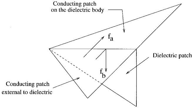
Fig. 5. Dielectric-conductor junction.
