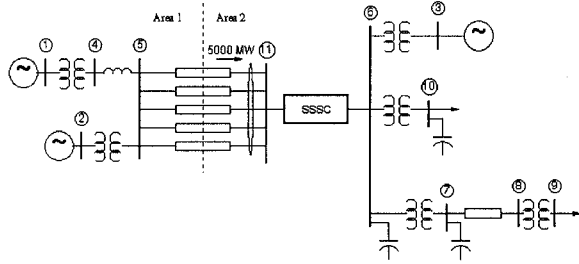
Figure 8 – Example System for Comparison of SSSC Controls
