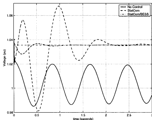
Figure 14 – Voltage at Area 2 Bus (- no control, -- StatCom, -.- StatCom/BESS)
