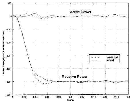
Figure 5 – Step Change in Reactive Power
