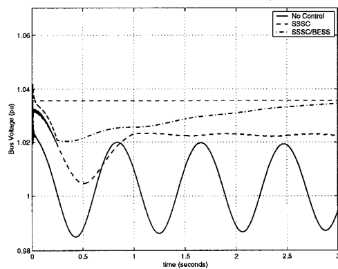
Figure 15 – Voltage at Area 2 Bus (- no control, -- SSSC, -.- SSSC/BESS)
