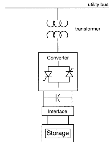
Figure 1 – Integrated StatCom with Energy Storage
