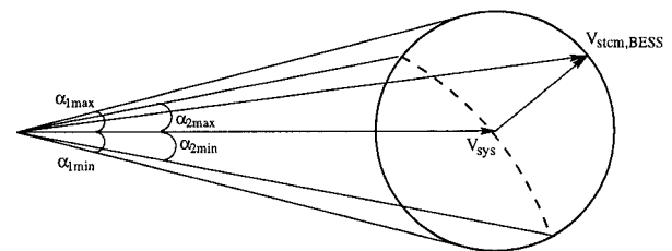
Figure 2 – StatCom/BESS Voltage Characteristics
