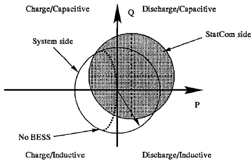
Figure 3 – StatCom/BESS Output Power Characteristics
