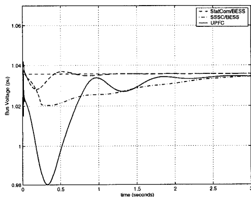
Figure 16 – Voltage at Area 2 Bus (- UPFC, -- StatCom/BESS, -.- SSSC/BESS)
