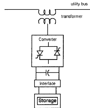
Figure 4 – Integrated SSSC with Energy Storage
