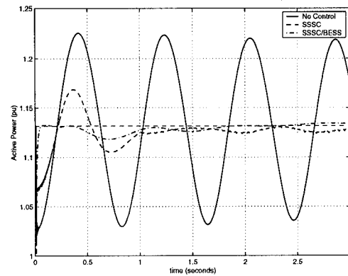
Figure 10 – Active Power Flow Between Areas (-no control, -- SSSC, -.- SSSC/BESS)
