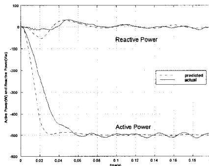
Figure 6 – Step Change in Active Power
