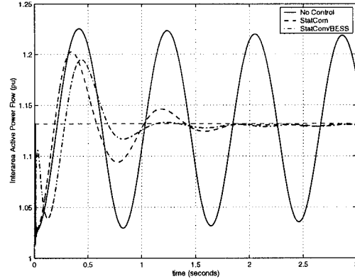
Figure 9 – Active Power Flow Between Areas (- no control, -- StatCom, -.- StatCom/BESS)
