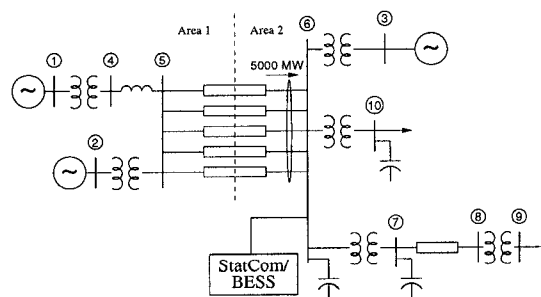
Figure 7 – Example System for Comparison of StatCom Controls
