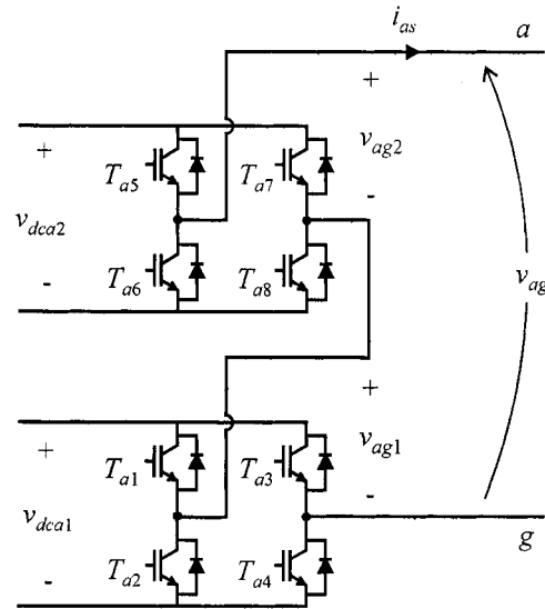
Fig. 2. Cascade-3/3H topology.
