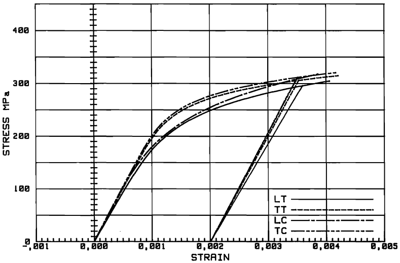
FIGURE 2 ANALYTICAL STRESS-STRAIN CURVES FOR STAINLESS STEEL TYPE 304
