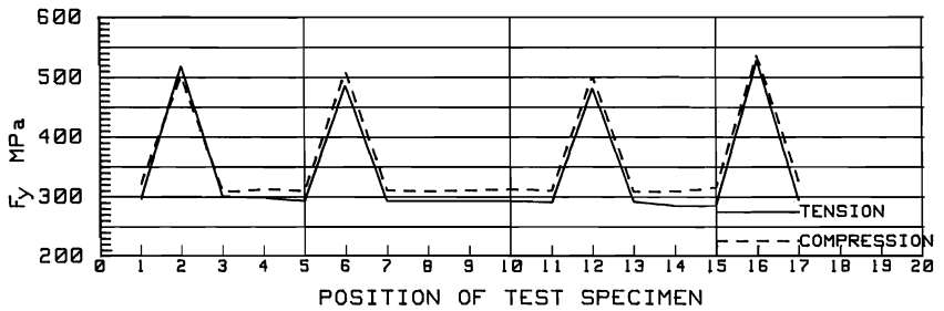
FIGURE 9 VARIATION OF MECHANICAL PROPERTIES FOR TYPE 3CR12 CORROSION RESISTING STEEL
