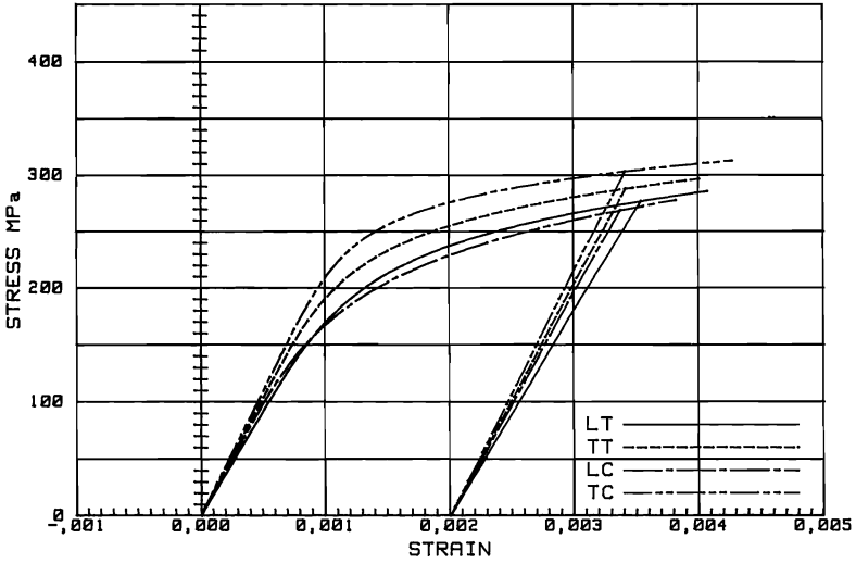
FIGURE 3 ANALYTICAL STRESS-STRAIN CURVES FOR STAINLESS STEEL TYPE 316
