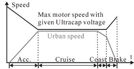
Fig. 7. UC source operating range in urban driving.
