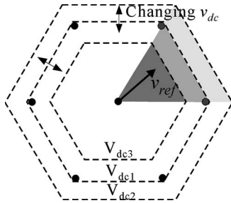
Fig. 4. New modulator space vector illustration.
