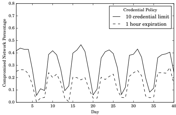
Figure 5: Daily simulation results for both credential policies.
