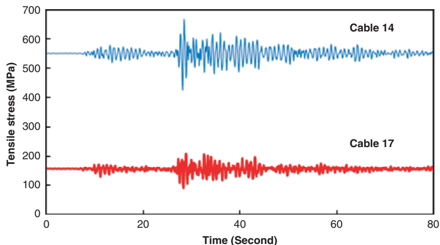
FIGURE 7 Time history of tensile stress in cables.
