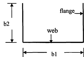
Figure 1 Plain Channel
