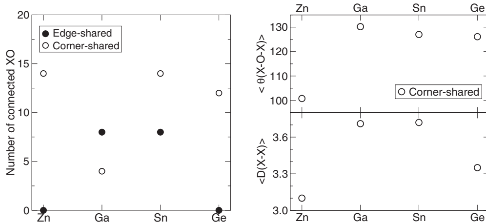
FIG. 9. (Left) Number of edge-shared and corner-shared X - X pairs in a -In- X -O. (Right) Average X - X distance, in Å, and average X -O- X angle, in degrees, for the XO_x polyhedra connected via corner sharing in amorphous In- X -O. The corresponding values for edge-shared X - X pairs for X = \text{Sn} and \text{Ga} are given in the text.
