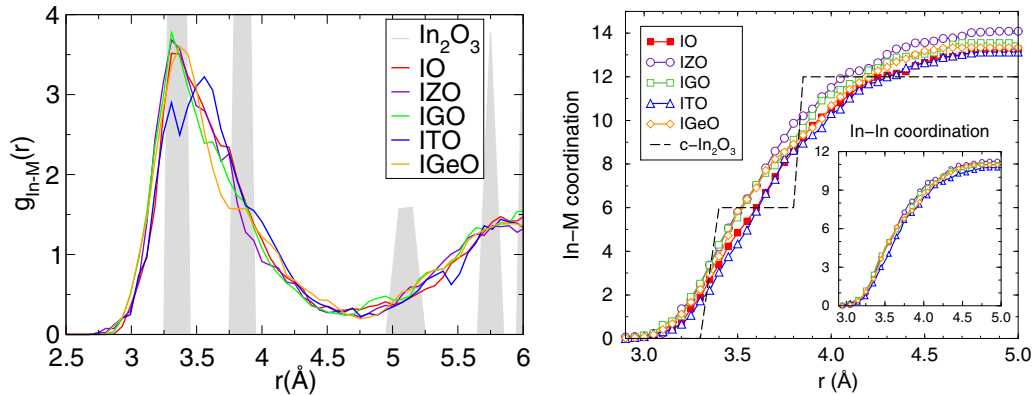
FIG. 6. (Color online) (Left) Radial In- M distribution function, g_{\text{In}-M}(r) , where M = \text{In} or X = \text{Zn}, \text{Ga}, \text{Sn}, \text{Ge} as a function of distance from an In atom in crystalline \text{In}_2\text{O}_3 and in amorphous In-O and In- X -O. (Right) Total In- M coordination, where M = \text{In} or X = \text{Zn}, \text{Ga}, \text{Sn}, \text{Ge} , as a function of distance from an In atom in crystalline \text{In}_2\text{O}_3 and in amorphous In-O and In- X -O. The inset shows the In-In coordination as a function of distance for the same.
