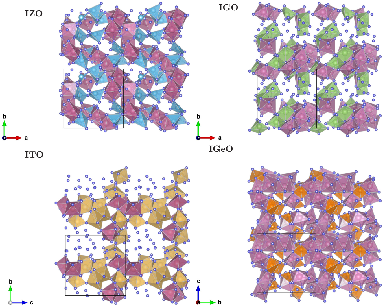
FIG. 12. (Color online) Atomic structures of a -In- X -O, X = \text{Zn} , Ga, Sn, or Ge, highlighting the \text{InO}_6 and \text{XO}_x polyhedra only. Small spheres represent oxygen atoms, and large spheres represent In or X atoms.
