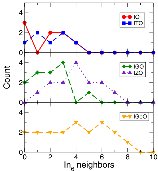
FIG. 10. (Color online) The number of In 6 neighbors calculated within a radial cutoff distance of 3.8 Å from a central In 6 in a -In-O and a -In-X-O. The oxides are grouped according to the fractional number of the six-coordinated In atoms, cf., Fig. 4, that is ~20% for a -In-O and a -ITO; ~30% for a -IGO, and a -IZO; and ~40% for a -IGeO.
