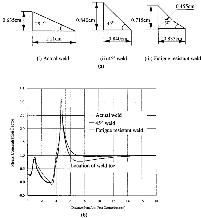
FIGURE 7 (a) Various weld profiles; (b) stress concentration factors.
