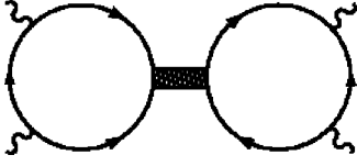
FIG. 3. Leading contribution to the \chi_{\text{off}}^{(4)} (see Appendix C).
