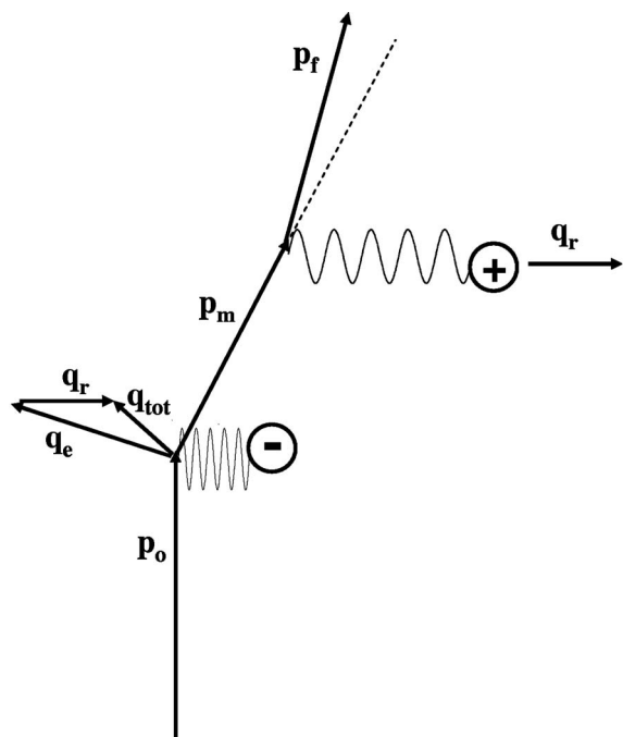
FIG. 4. Schematic diagram of the higher-order mechanism involving elastic scattering of the projectile by the residual target ion. p_0 , p_m , and p_f are the initial, intermediate, and final projectile momenta, respectively, and q_e , q_r , and q are the momentum transfers to the electron and recoil ion and the total momentum transfer.
