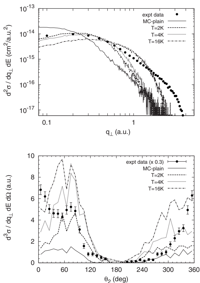
FIG. 4. Double differential (top) and fully differential (bottom) cross sections for single ionization of helium by 3.6 MeV/u Au 53+ for an energy of the ejected electron E_e = (10 \pm 3) eV. The FDSC is displayed in the scattering plane for a momentum transfer of q_{\perp} = (1 \pm 0.3) a.u.
