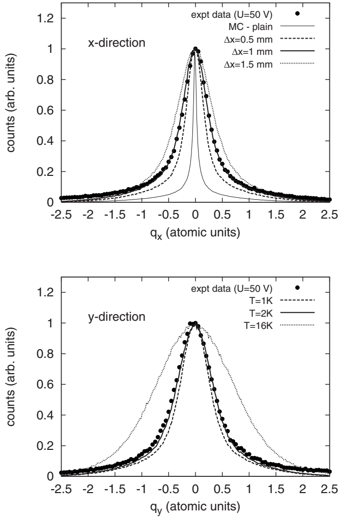
FIG. 5. Single differential cross sections for 100 MeV/ u C^{6+} single ionization of helium for the x (top) and y direction (bottom). Points: Experimental data, lines: Monte Carlo simulation results.
