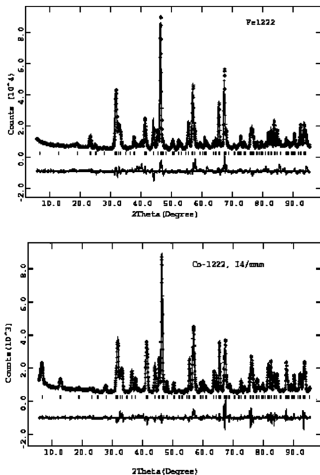
FIG. 1. Observed and fitted neutron diffraction patterns for \text{MSr}_2(\text{Y}_{3/4}\text{Ce}_{1/4})_2\text{Cu}_2\text{O}_z ( M = \text{Fe, Co} ).
