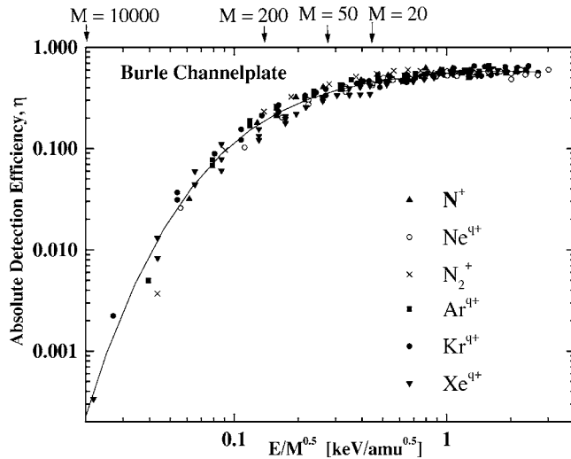
FIG. 3. Absolute ion detection efficiencies for a channelplate. The efficiencies are plotted vs the impact energy divided by the square root of the ion mass. The solid line is a polynomial fit to all the data. Arrows on the top axis indicate values of the abscissa for detecting singly charged positive ions of various masses if the front plate is biased at -2 kV and the backplate of a chevron pair is grounded as is often used for channelplate pairs.
