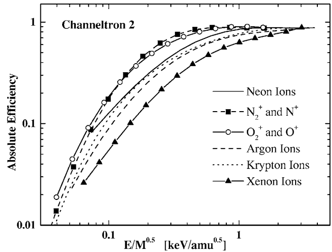
FIG. 4. Ion detection efficiencies measured for CEM 2. Lines and lines with symbols representing polynomial fits to the data for each ion species are shown rather than individual data points.
