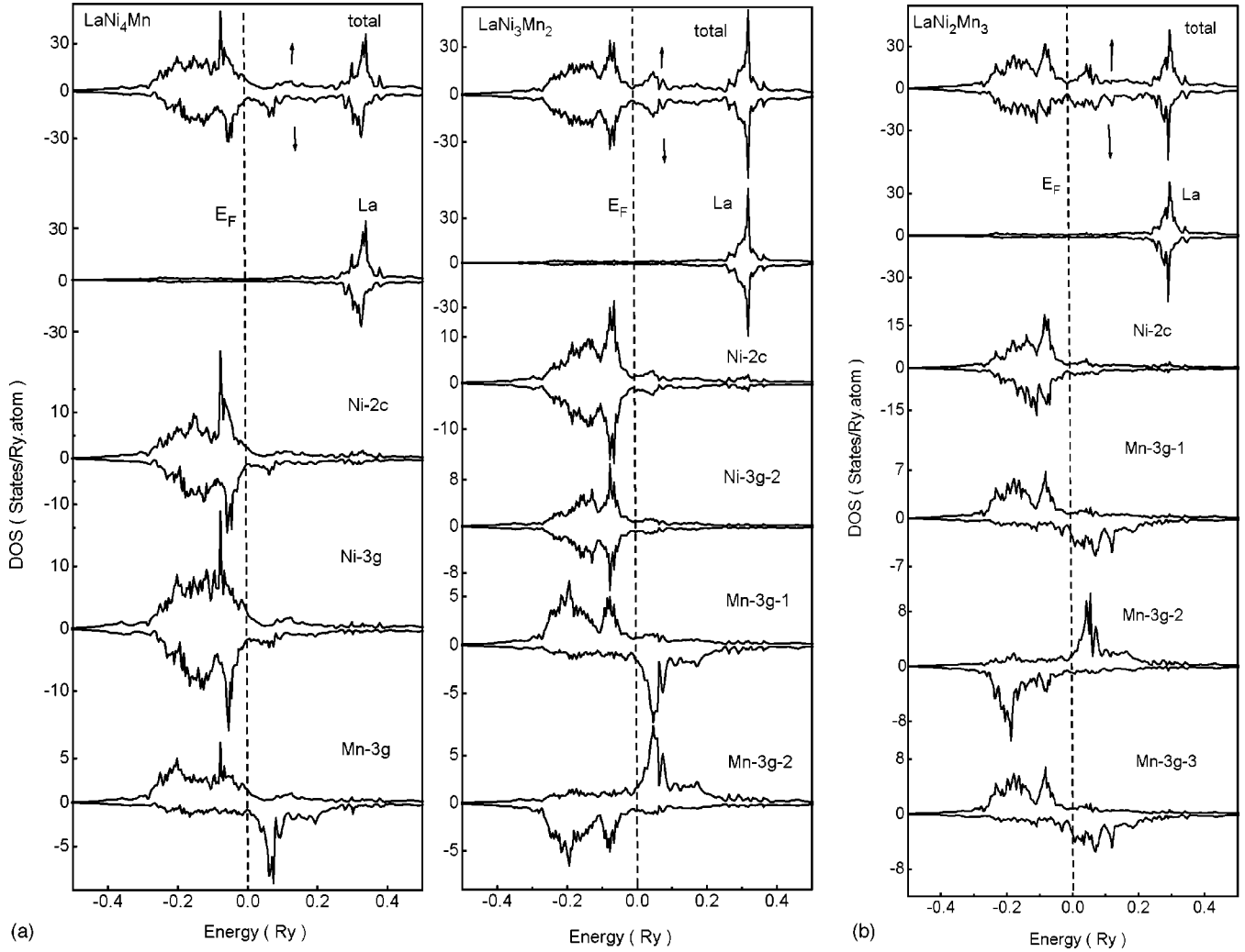
FIG. 8. Total densities of states of \text{LaNi}_{5-x}\text{Mn}_x ( x=1.0, 2.0, \text{ and } 3.0 ).
