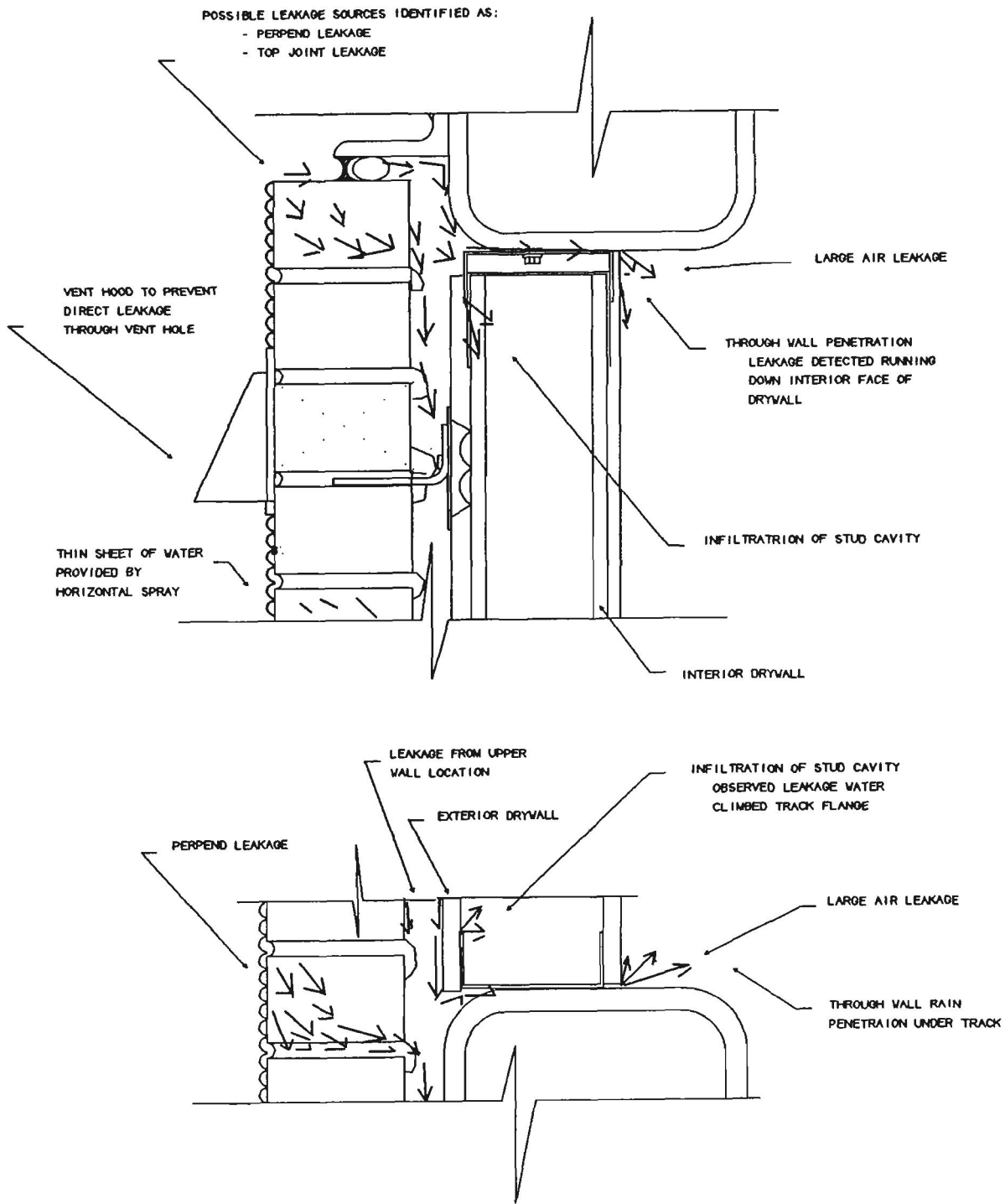
FIGURE 4.11 OBSERVED LEAKAGE PATHS DURING TESTING WITH SUB-STANDARD PERIMETER SEALING OF THE AIR BARRIER IN WALL
