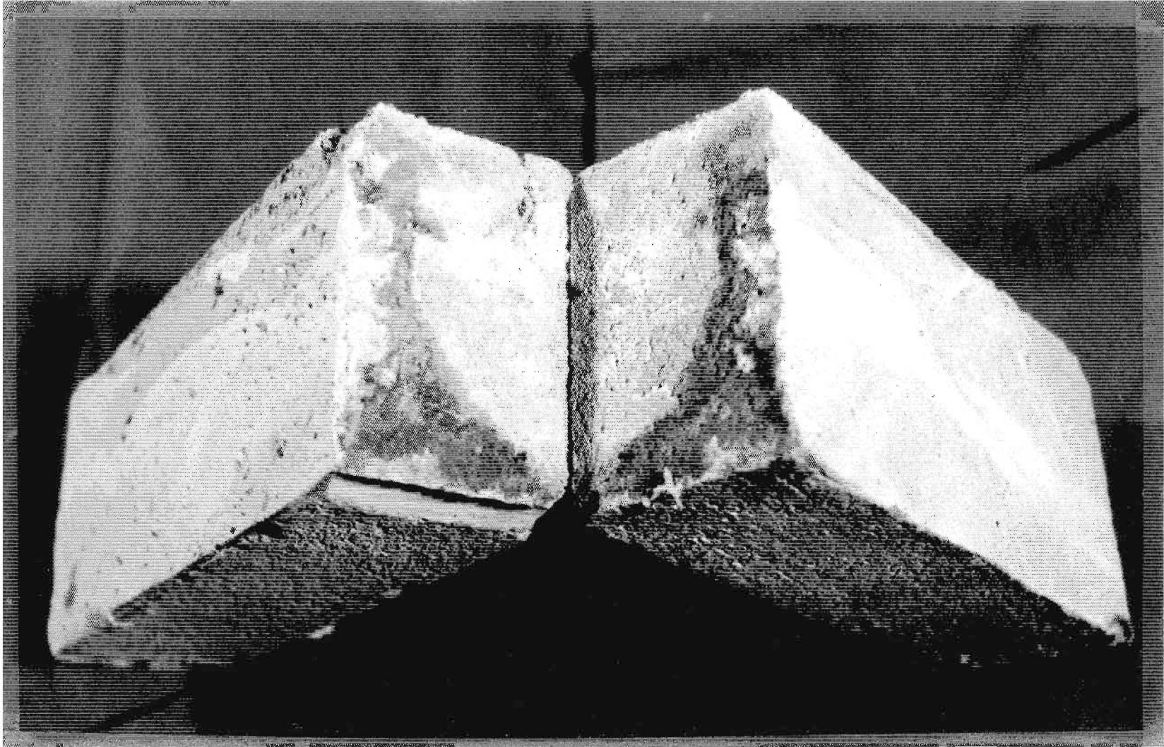
FIGURE 4.7 DYE PATTERN IN A HEAD JOINT (DEPRESSURIZED CAVITY CONDITION)
