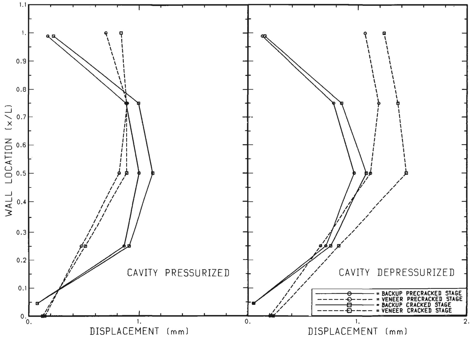
FIGURE 5.9 (b) DISPLACEMENTS FOR WALL2 BEFORE AND AFTER CRACKING OF THE BRICK VENEER
