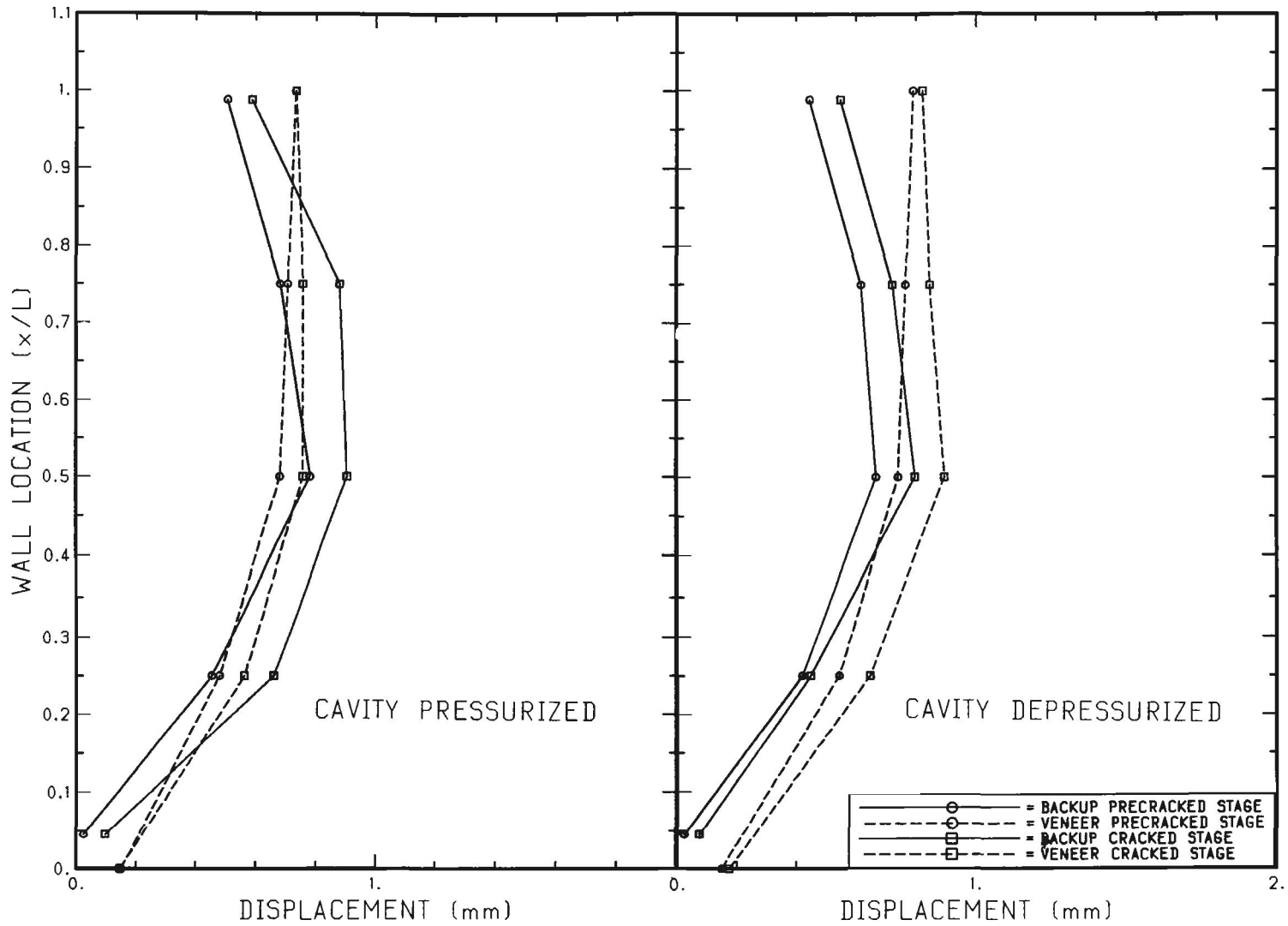
FIGURE 5.9(d) DISPLACEMENTS FOR WALL4 BEFORE AND AFTER CRACKING OF THE BRICK VENEER
