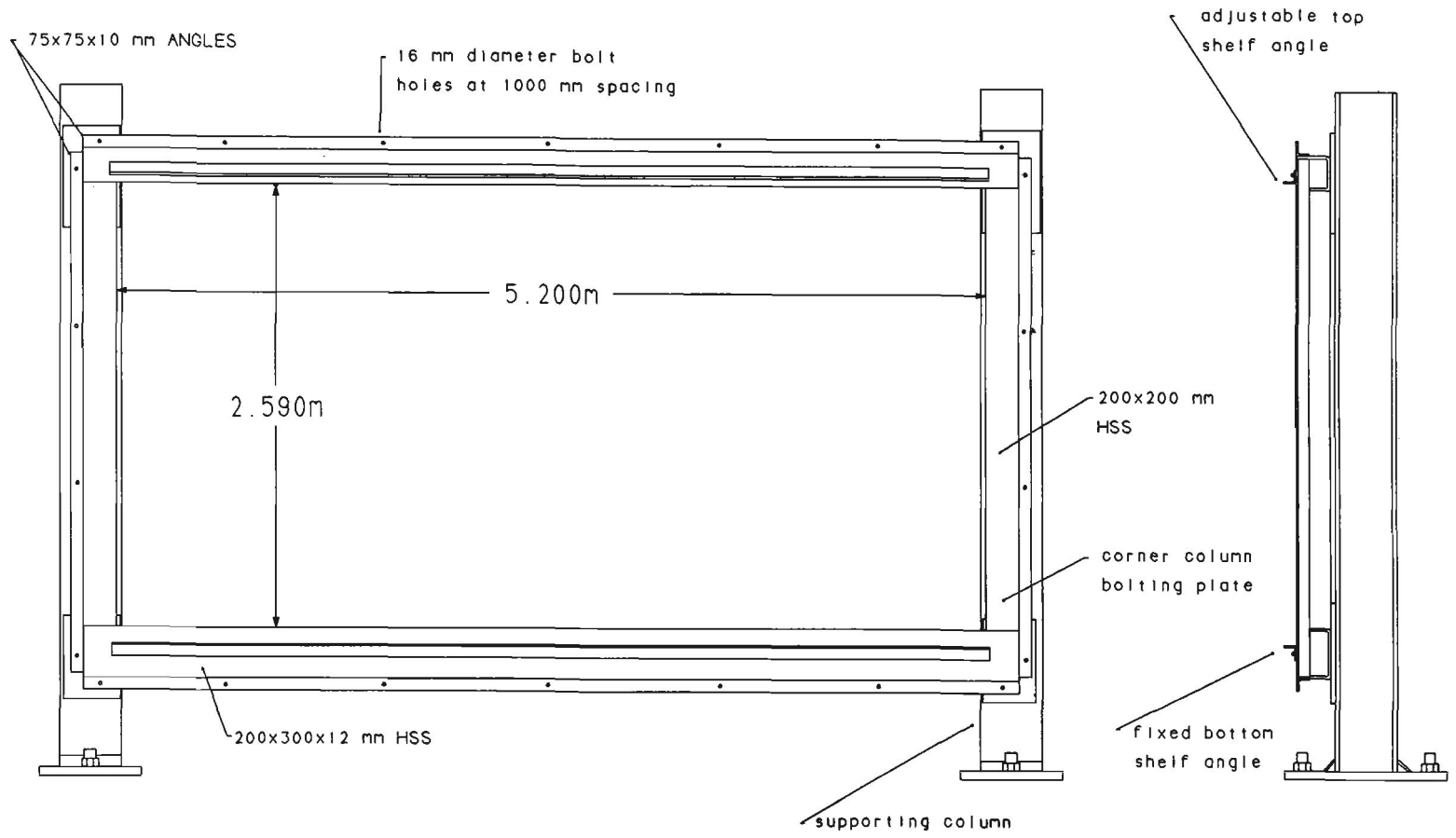
FIGURE 2.2 SPECIMEN FRAME
