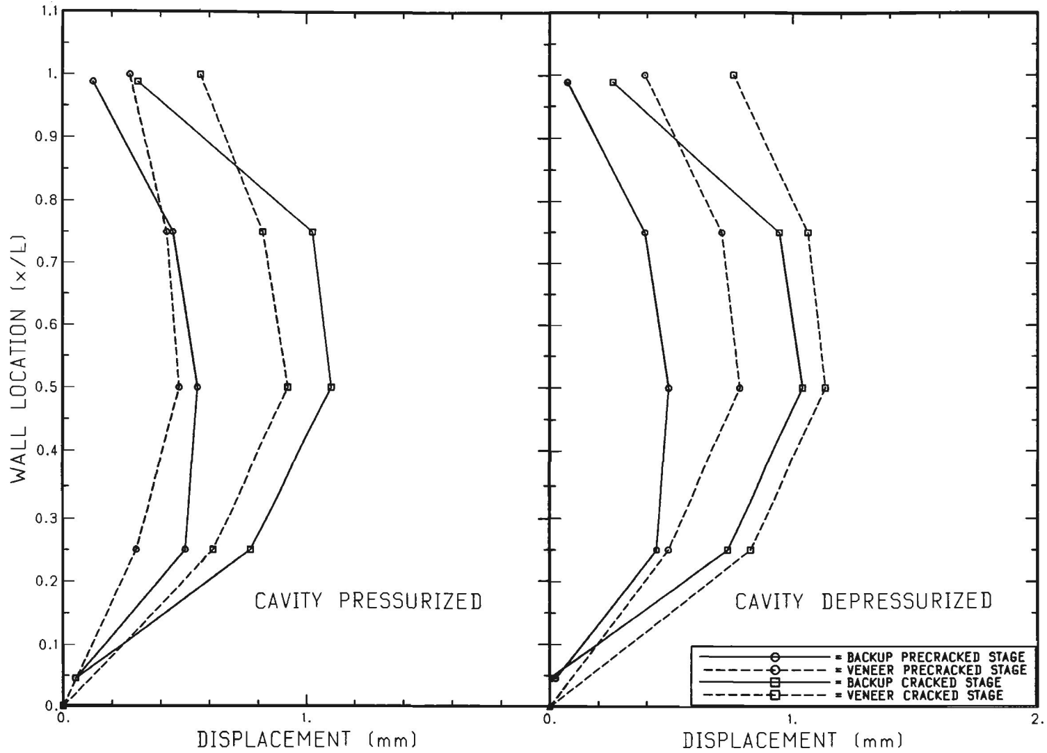
FIGURE 5.9(a) DISPLACEMENTS FOR WALL1 BEFORE AND AFTER CRACKING OF THE BRICK VENEER
