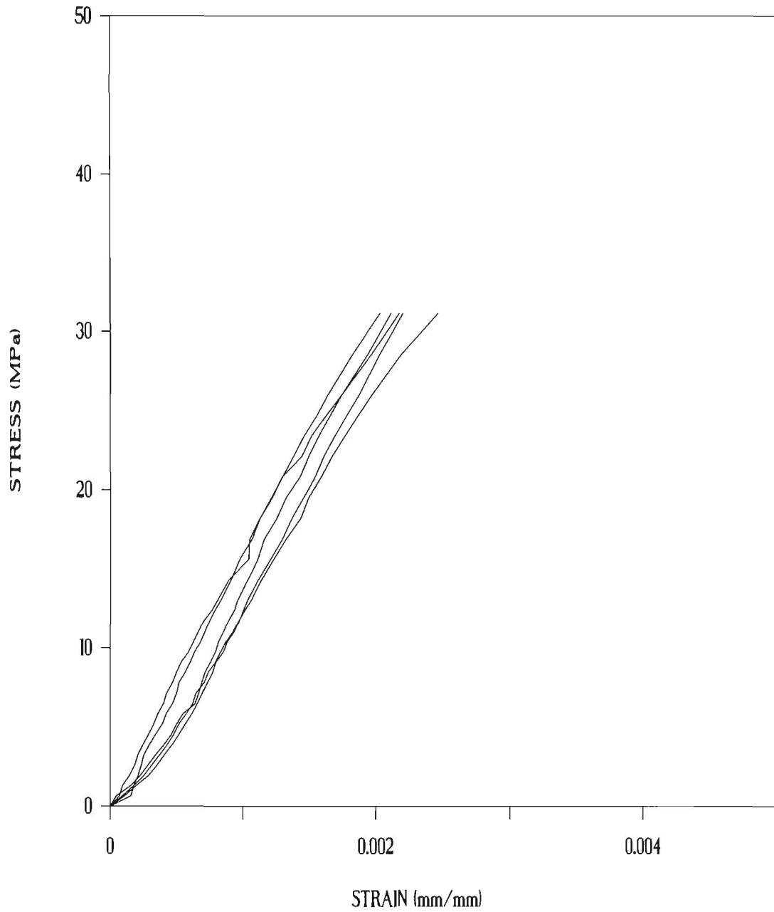
FIGURE A1.1 STRESS STRAIN CURVES - WALL1 PRISMS
