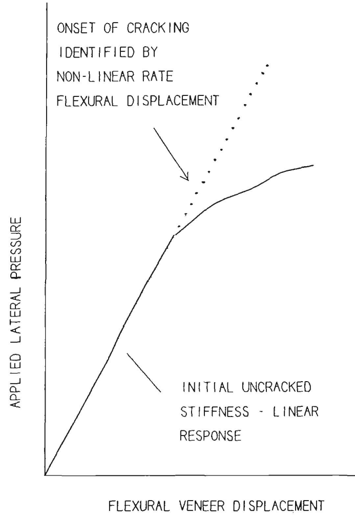
FIGURE 2.20 GRAPHICAL IDENTIFICATION OF ONSET OF VENEER CRACKING
