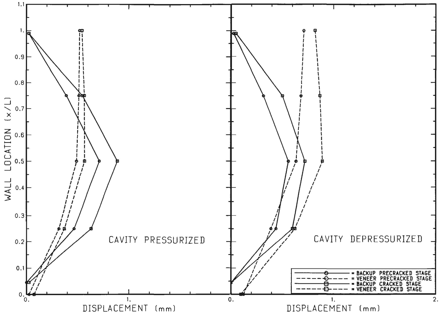
FIGURE 5.9(c) DISPLACEMENTS FOR WALL3 BEFORE AND AFTER CRACKING OF THE BRICK VENEER
