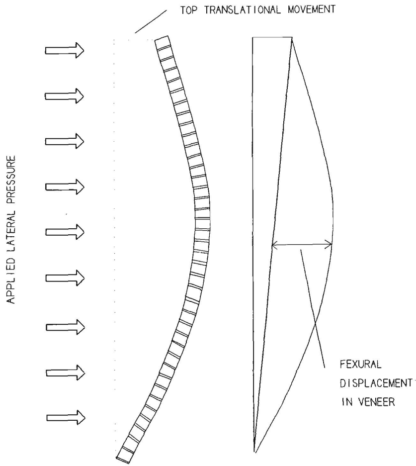
FIGURE 2.19 FLEXURAL DISPLACEMENT IN VENEER
