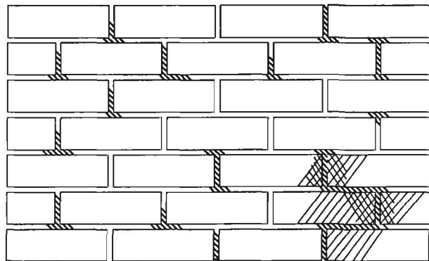
FIGURE 4.2 PROGRESS OF DAMPNES IN JOINTS DURING THE CAVITY PRESSURIZED TEST OF WALL3
