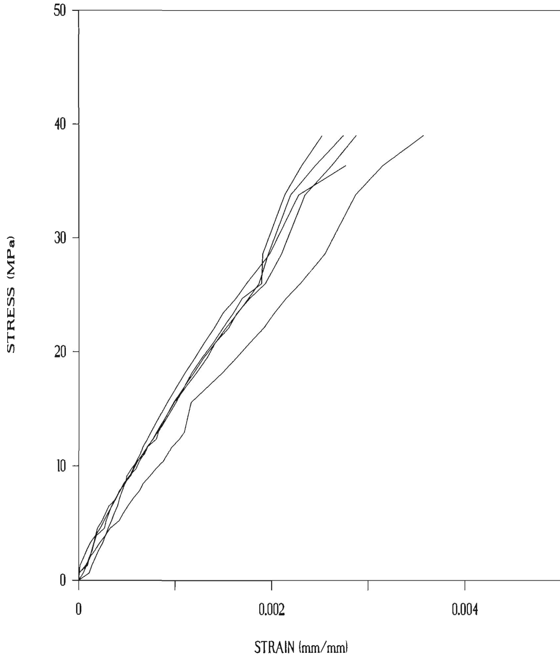
FIGURE A1.2 STRESS STRAIN CURVES - WALL2 PRISMS
