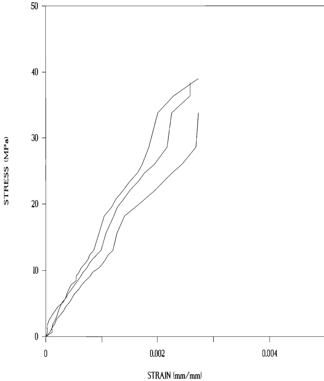
FIGURE A1.3 STRESS STRAIN CURVES - WALL3 PRISMS
