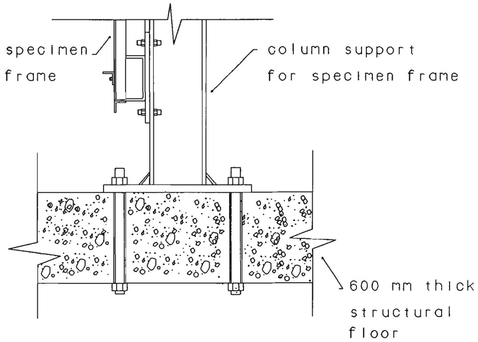
FIGURE 2.3 BASE CONNECTION
