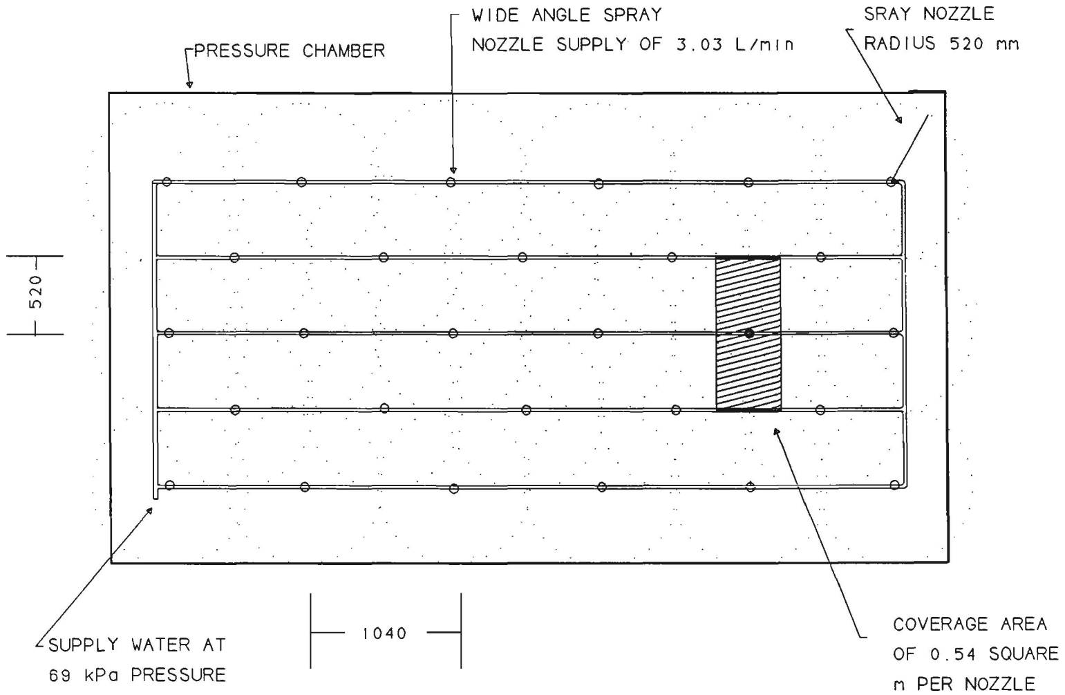
FIGURE 2.12 LAYOUT OF SPRAY NOZZLE SYSTEM
