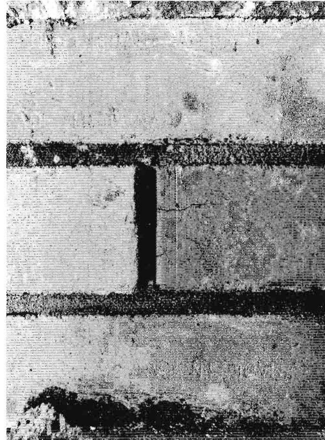
b) Half Empty Head Joint Heavily Contributing to Leakage
