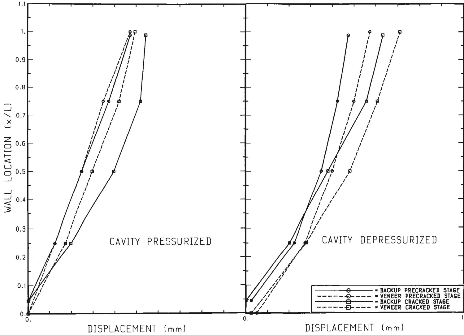
FIGURE 5.10 DISPLACEMENTS FOR WALL5 BEFORE AND AFTER CRACKING OF THE BLOCK BACKUP WALL
