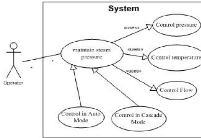
Figure 5. Use case Diagram for a plant control process
