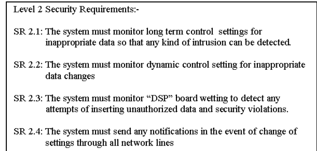
Figure 11: Security requirements for 'UPFC Facts Device' object
