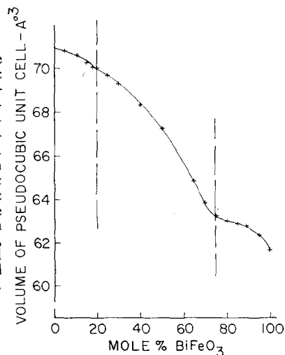
FIG. 3. Volume of the pseudocubic unit cell for \text{PbZrO}_3\text{-BiFeO}_3 solid solutions at room temperature as a function of composition. The change from the antiferroelectric to the ferroelectric orthorhombic phase shows little effect on the unit-cell volume, despite a pronounced effect on individual dimensions (see Fig. 2).
