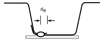
Figure C-D1-3 Nestable Side-Lap
