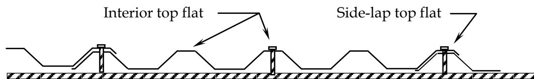
Figure D1.1.4.3-1 Fasteners Through Top Flat
