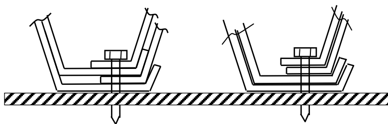
Figure C-D1.1.1-1 Examples of Connection With Four Thicknesses
