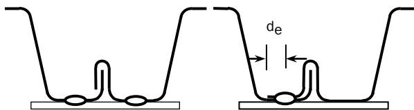
Figure C-D1-2 Interlocking Side-Laps
