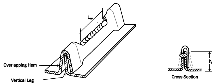
(a) Vertical Leg and Overlapping Hem Joint
