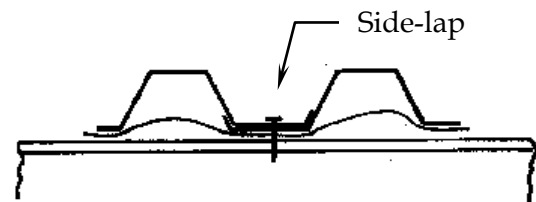
Figure D1.3-3 Fasteners at Lap-Down
