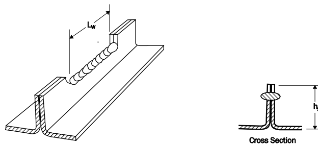
(b) Back-to-Back Vertical Leg Joint
