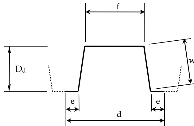
Figure 1.4-1 Panel Configuration
