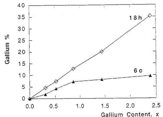
FIG. 2. Compositional dependence of the gallium site occupancy of \text{Ce}_2\text{Fe}_{17-x}\text{Ga}_x solid solution.
