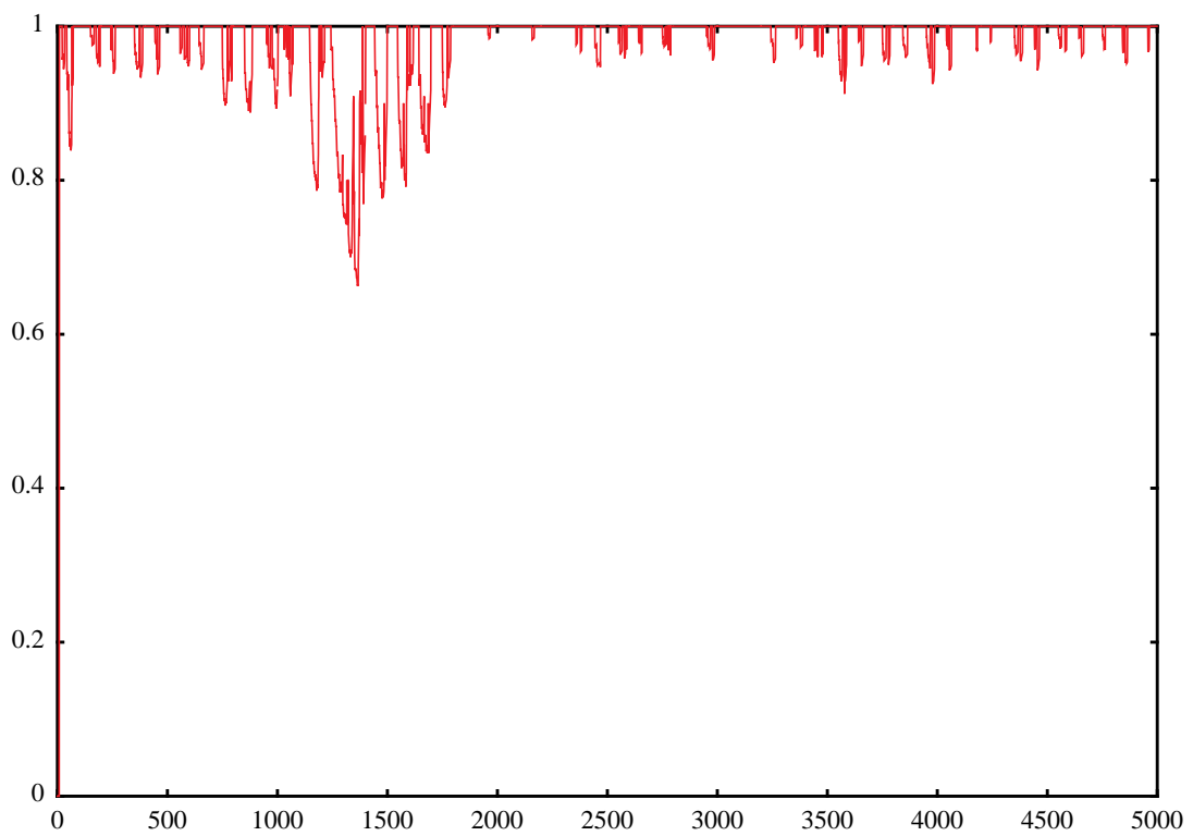
Figure 5.1.3c2. Three newsgroup experiment: Highest fitness values
