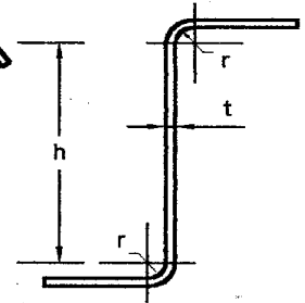
Unstiffened Flanges
