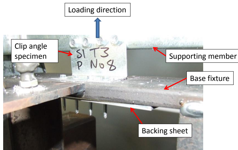
Figure 4.1: Close-up view of the pull-over test setup
