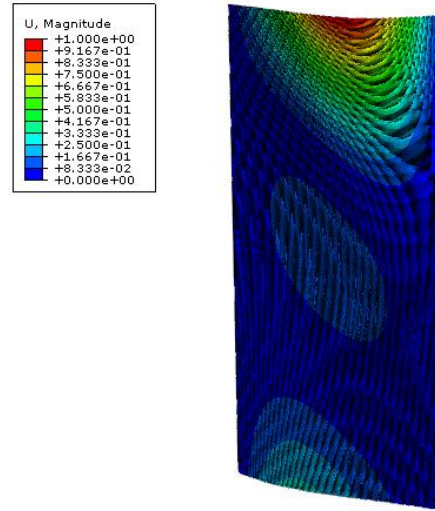
Figure 2.11: ABAQUS result
