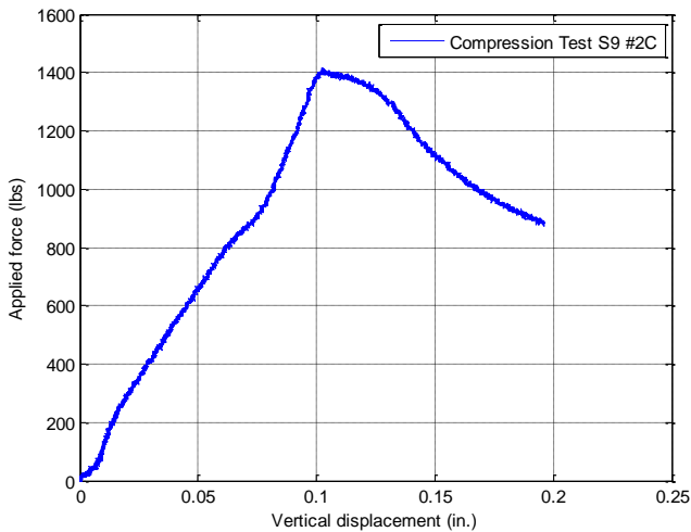
Figure 3.4: Test results of S9 #2C
