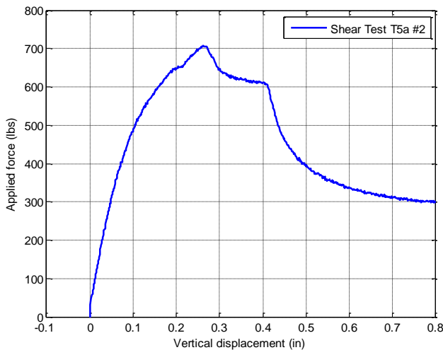
Figure 2.4: Test result of clip angle T5a #2
