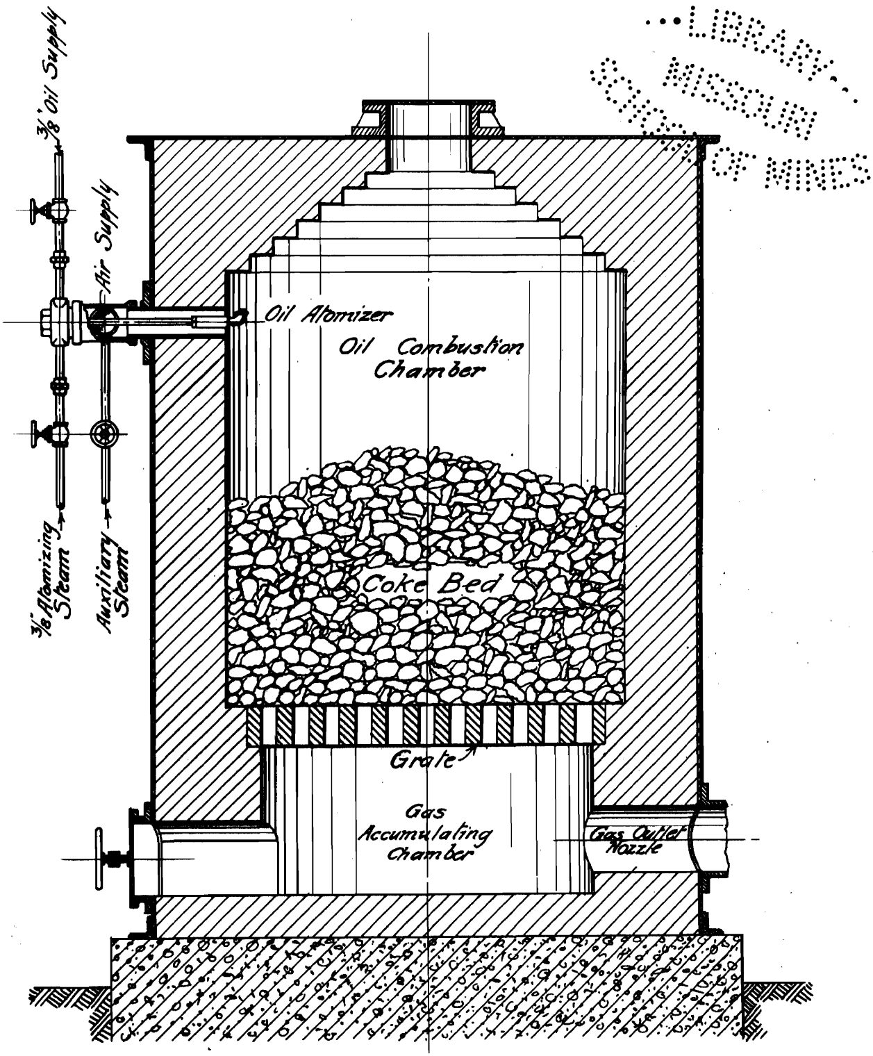
SECTIONAL ELEVATION.
