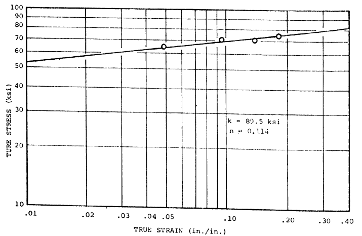
FIG. 11. TENSILE STRESS-STRAIN CURVE FOR STRAIN AGED SPECIMENS IN TERMS OF TRUE STRESS AND TRUE STRAIN.
