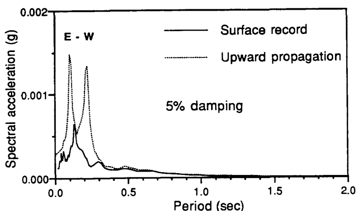
Figure 12: Spectral acceleration comparison between the EGF 93031 surface record and the SHAKE-based estimate of that surface record using as input the total motion record from bedrock.
